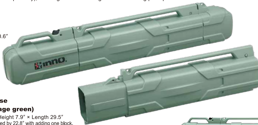
Rod Case J unit total length 40.6". Storable rod length: 39.8"
