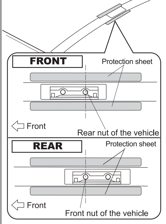
Fig-1 Carrier installation locations
